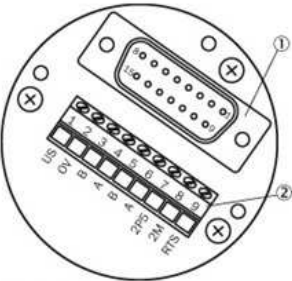
① = Internal plug connection to the encoder ② = External connection to the bus
