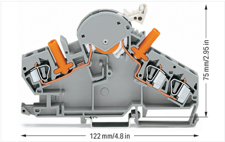
Voltage transformer terminal block, 282 Series, gray
